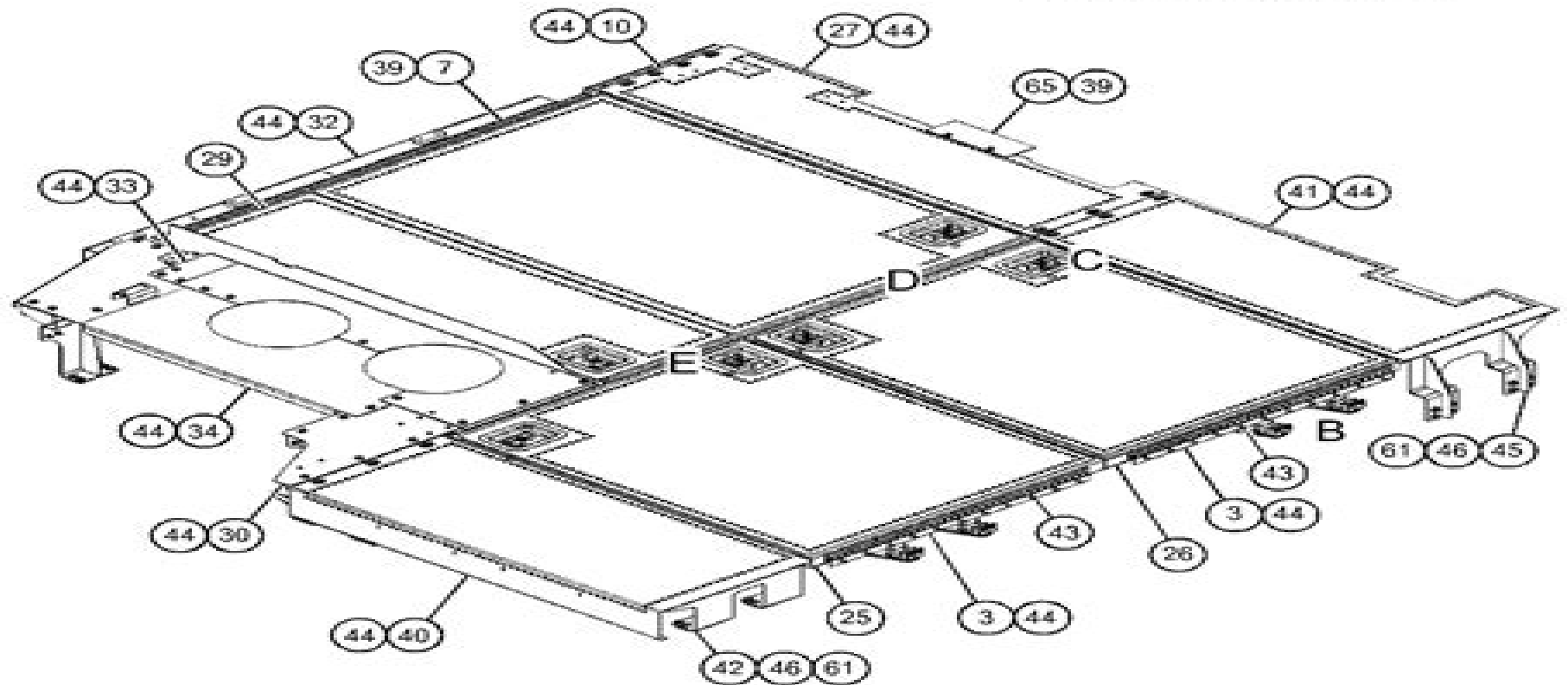
VIEW OF AREA A
