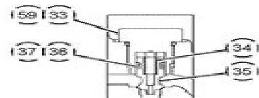
SECTION K-K
