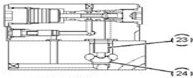
SECTION N-N
