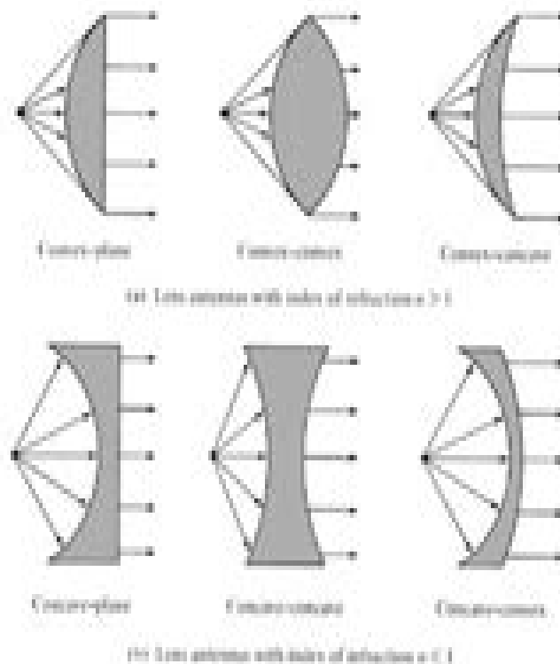
Figure 1.8 Typical lens antenna configurations. (source: L. V. Blake, Antennas , Wiley, New York, 1966).
